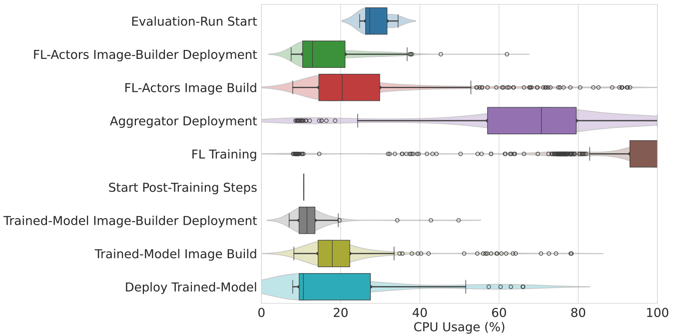
Figure C.4.: Experiment 2: CPU Utilization per Stage
