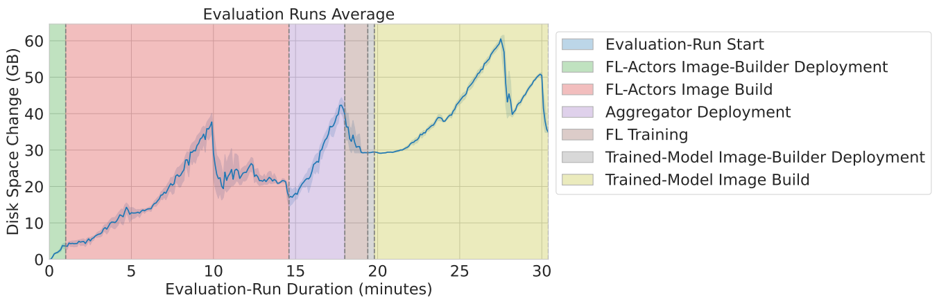
Figure 5.16.: Experiment 5: Disk Space
