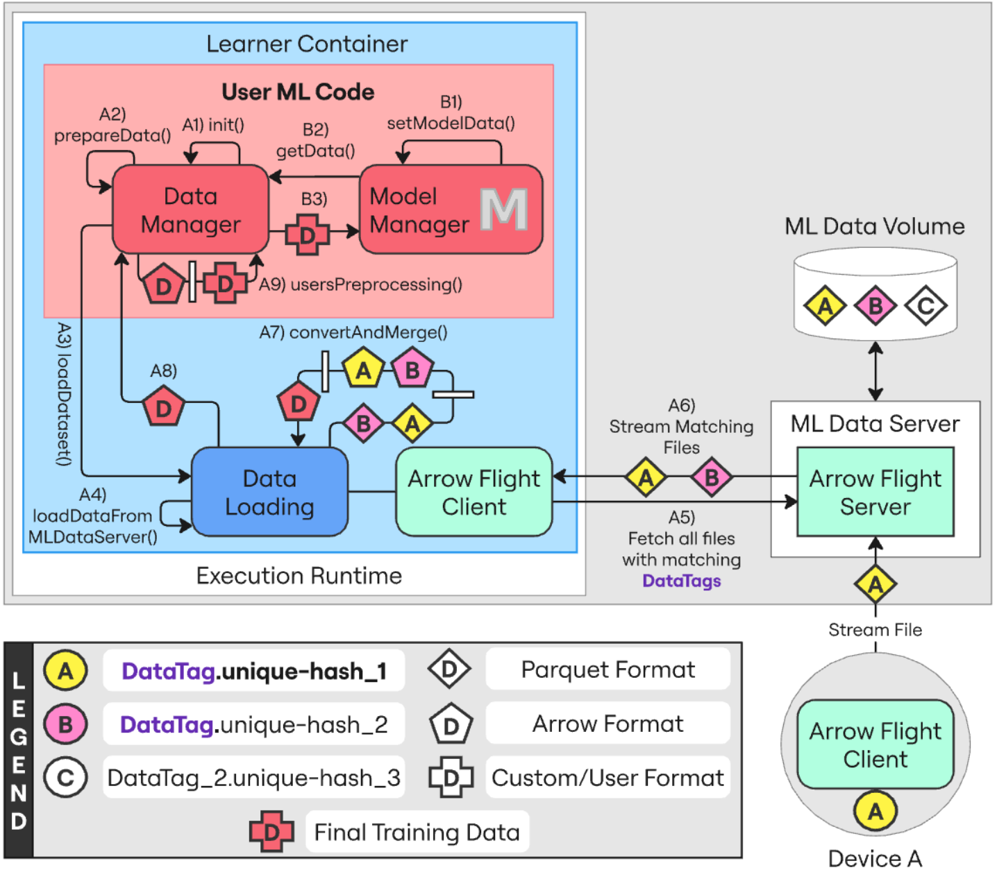
Figure 4.3.: Detailed FLOps Local Data Management Structure
