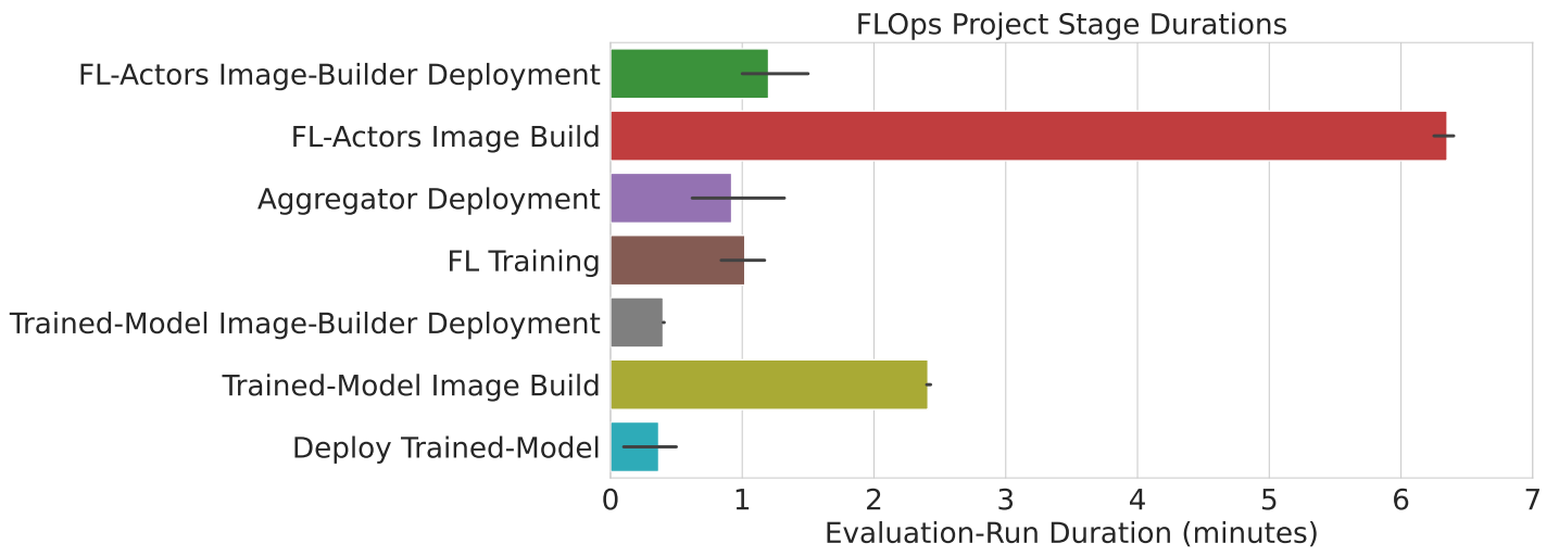
Figure 5.7.: Experiment 1: Stage Durations
