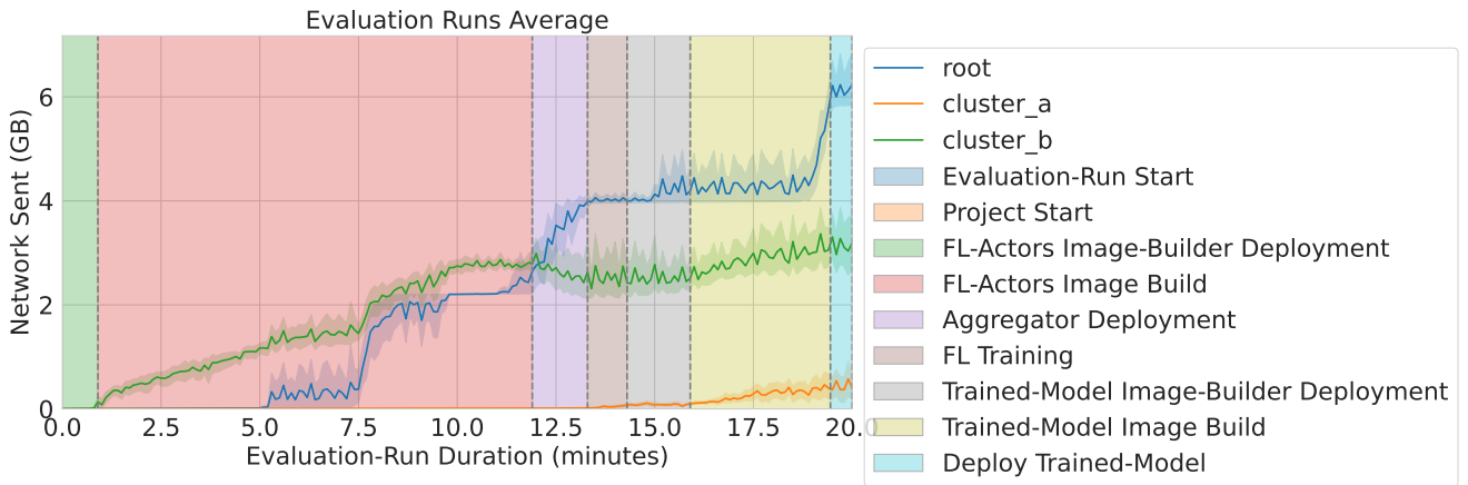
Figure 5.22.: Experiment 7: Send Network
