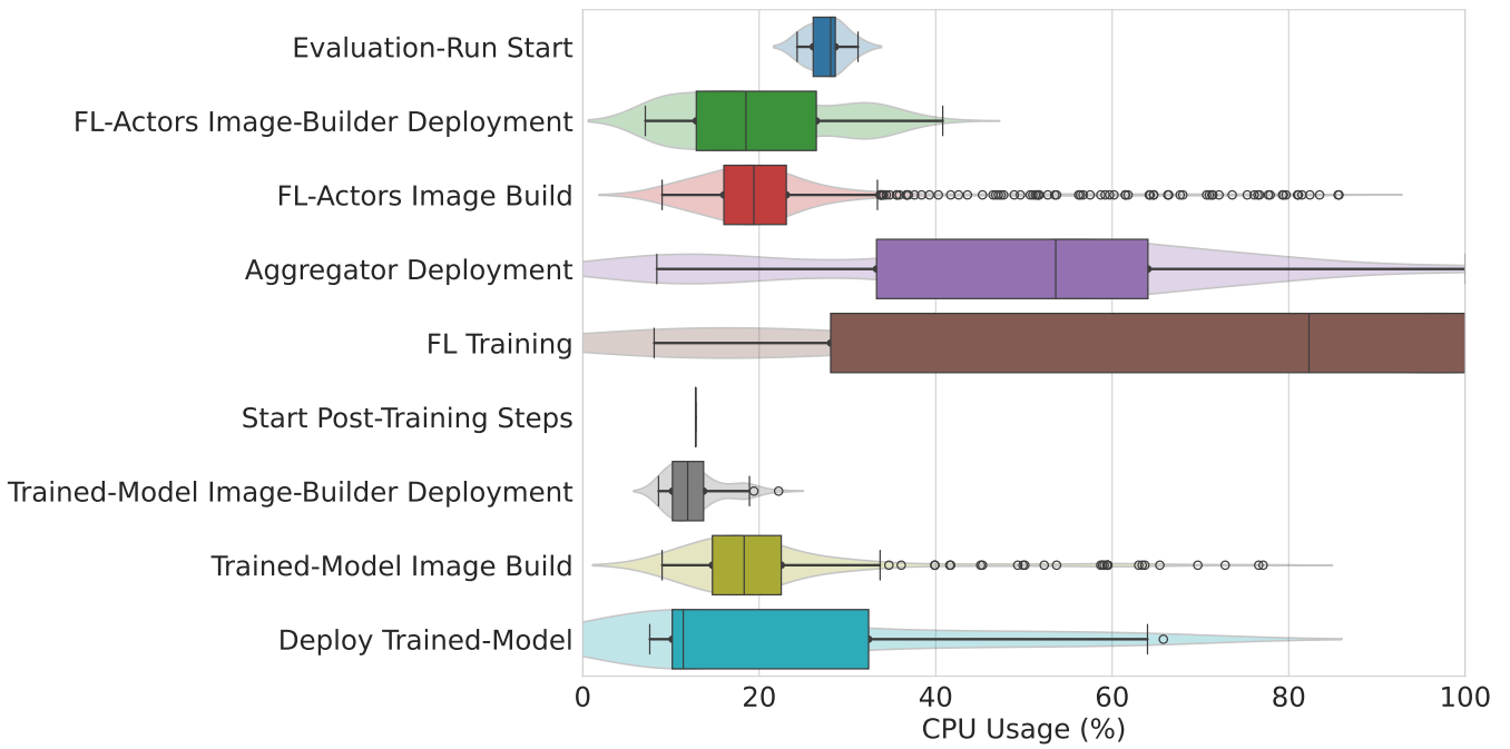
Figure 5.2.: Experiment 1: CPU Utilization by Stage
