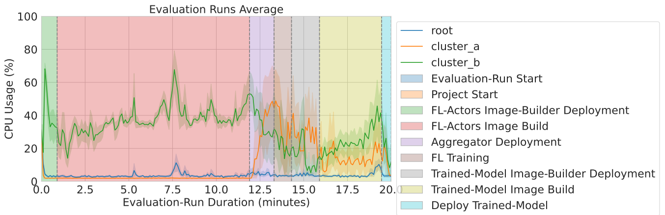
Figure 5.18.: Experiment 7: CPU Utilization
