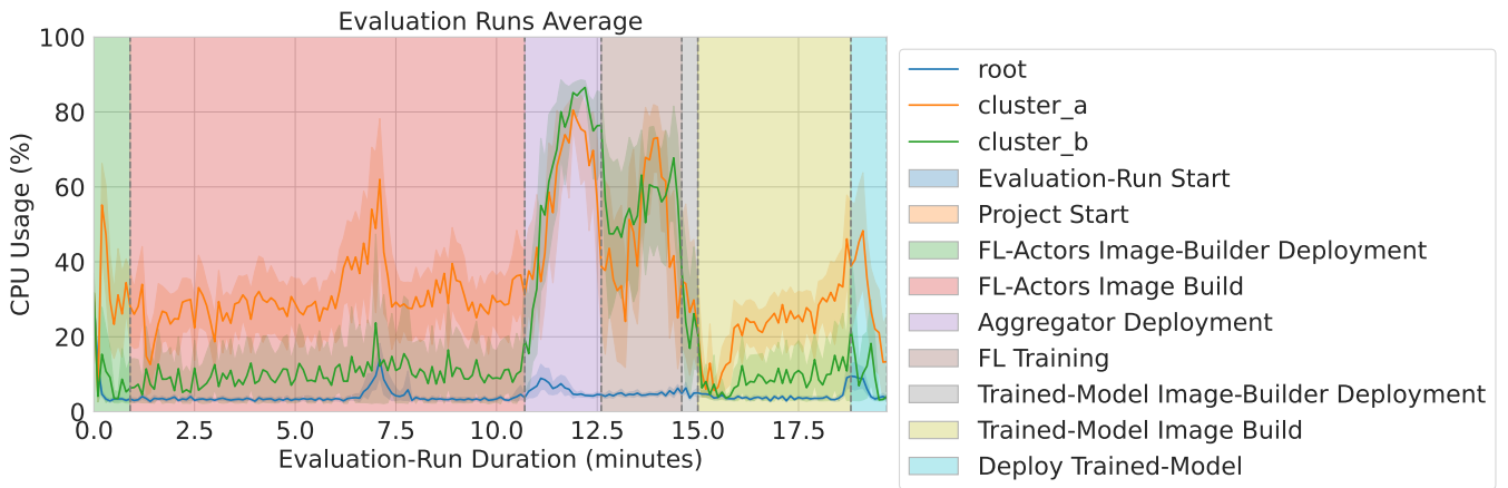
Figure 5.25.: Experiment 8: Multi-Cluster HFL CPU Utilization
