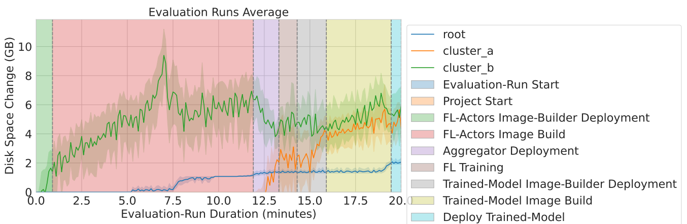
Figure 5.19.: Experiment 7: Memory Utilization
