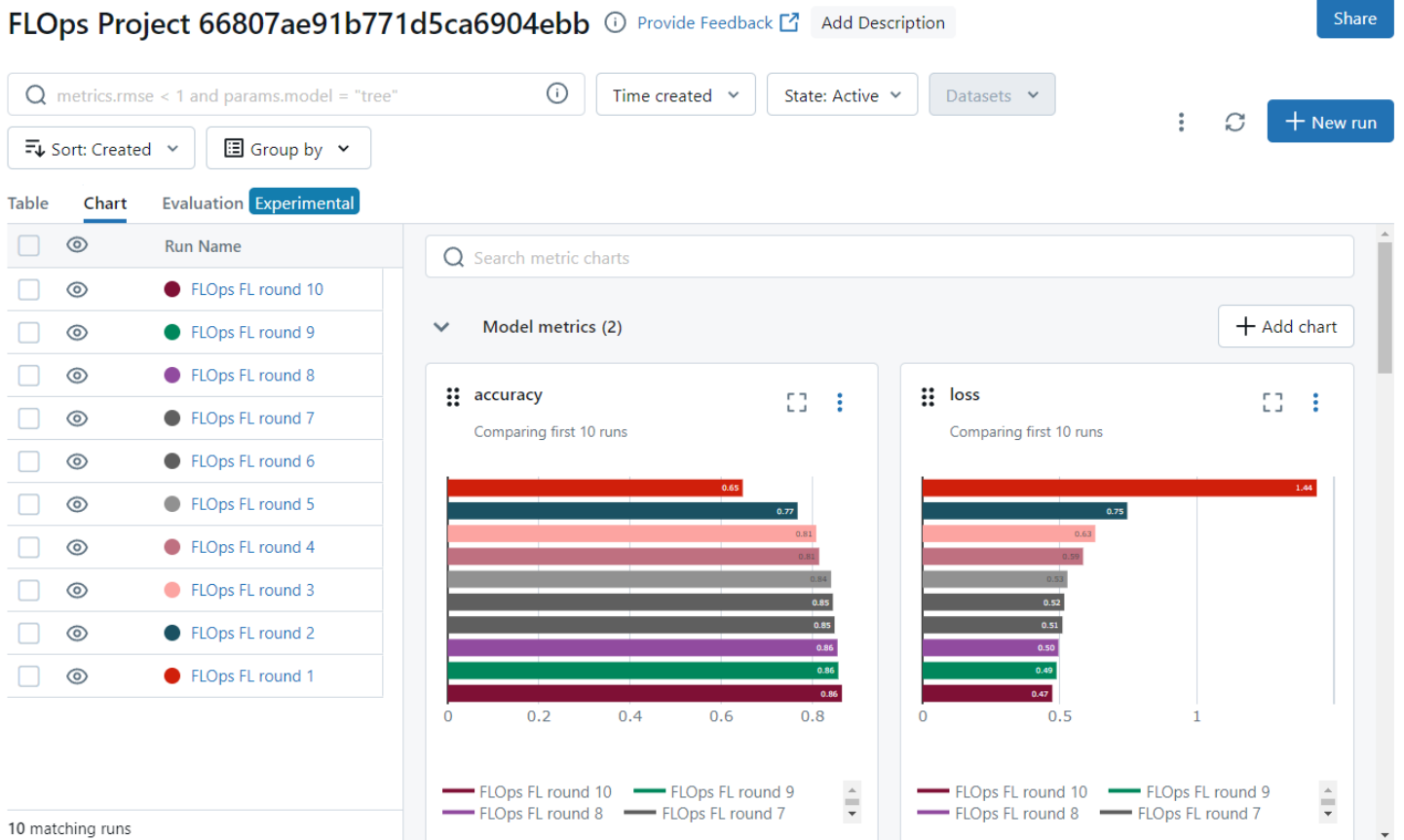
Figure 4.7.: MLflow's GUI Screenshot - Experiment Details
