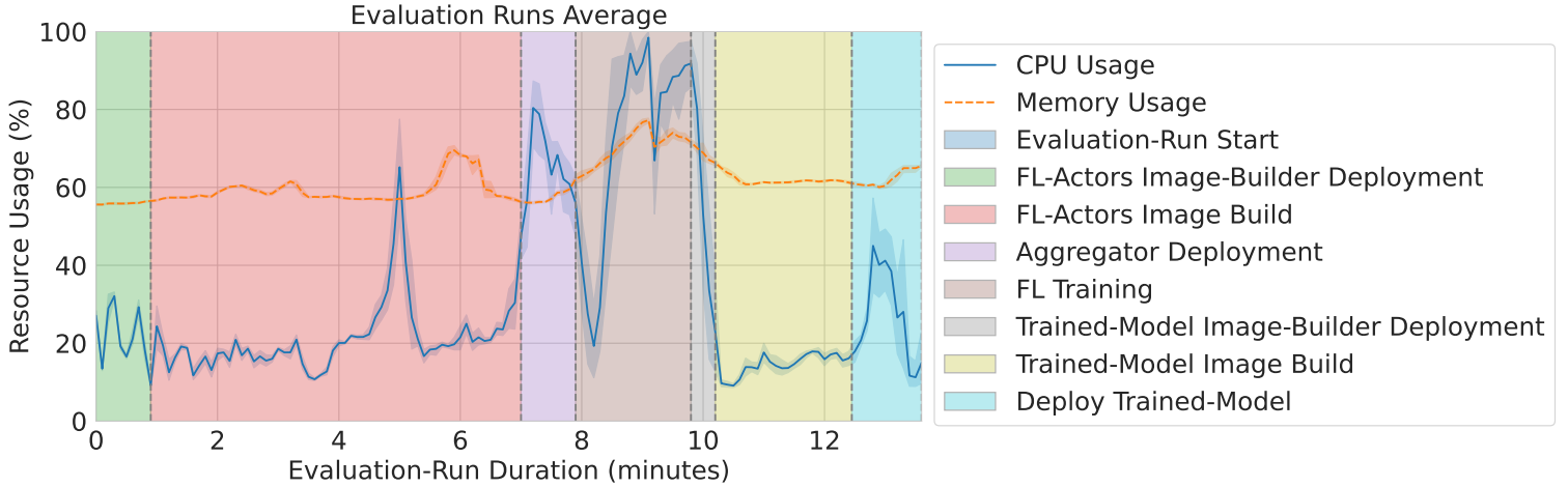
Figure 5.24.: Experiment 6: Monolith HFL CPU & Memory
