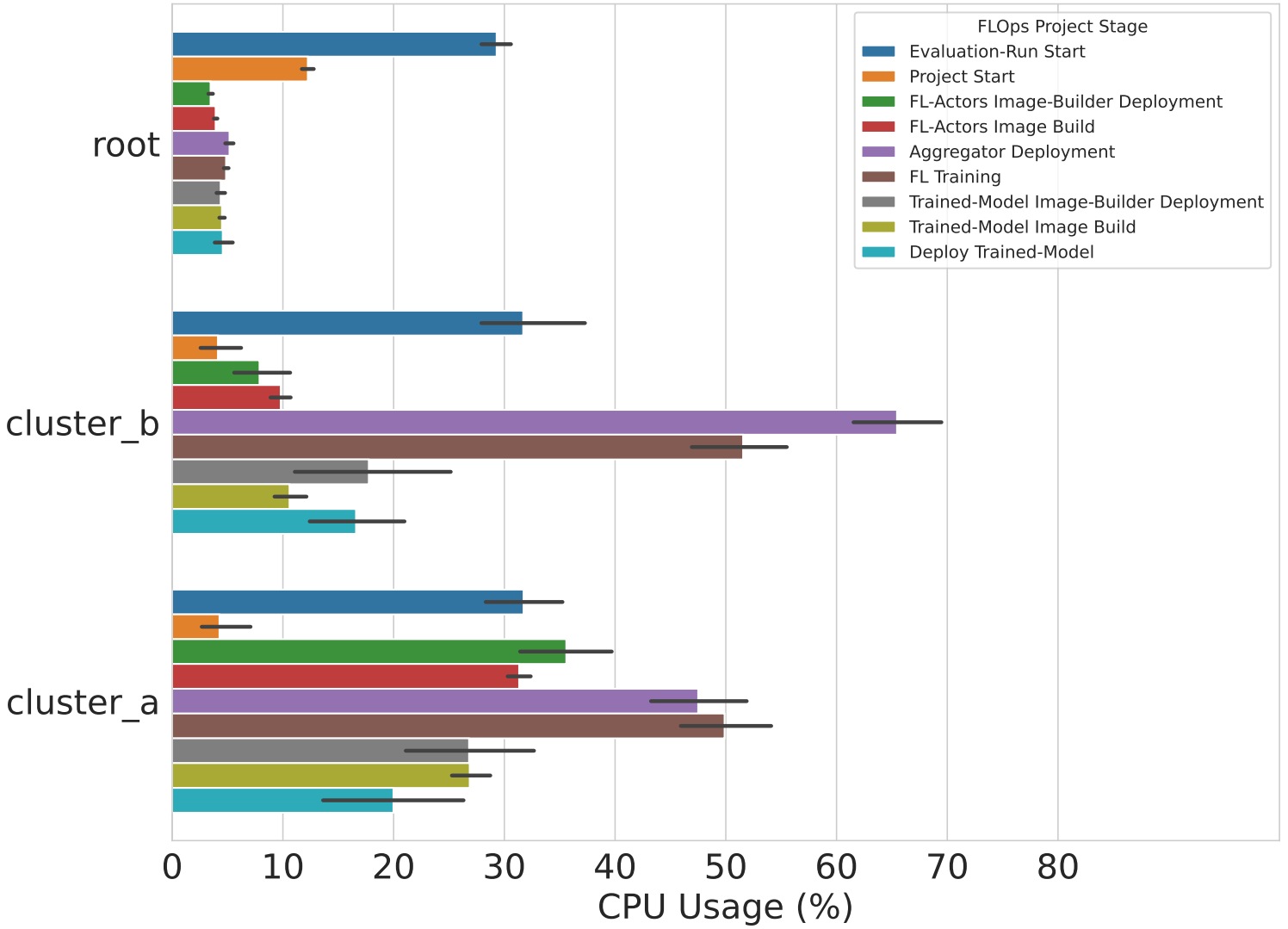
Figure C.12.: Experiment 8: CPU Utilization per Stage
