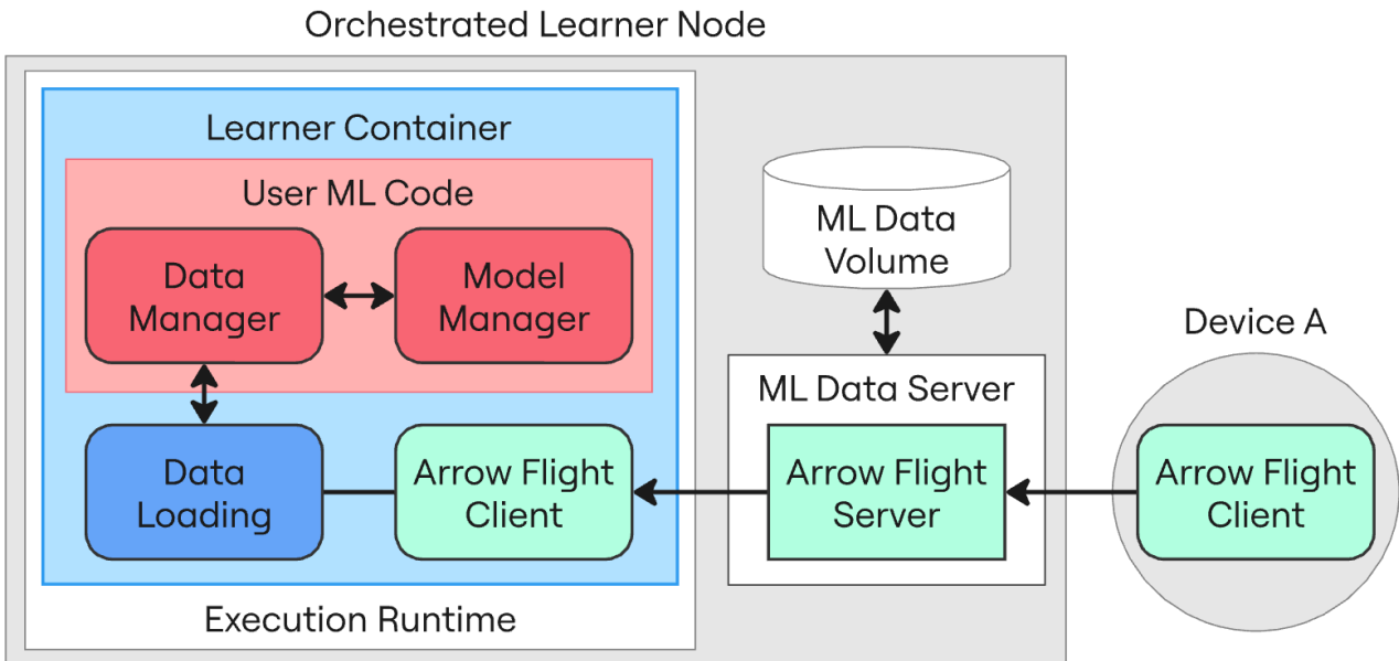
Figure 4.2.: FLOps Local Data Management Structure
