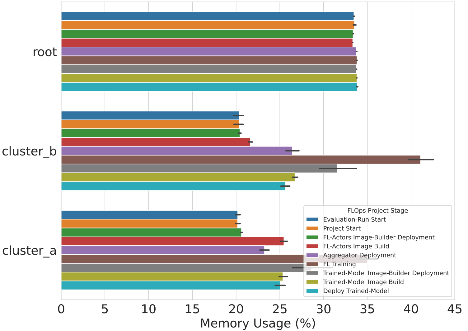
Figure C.13.: Experiment 8: Memory Utilization per Stage
