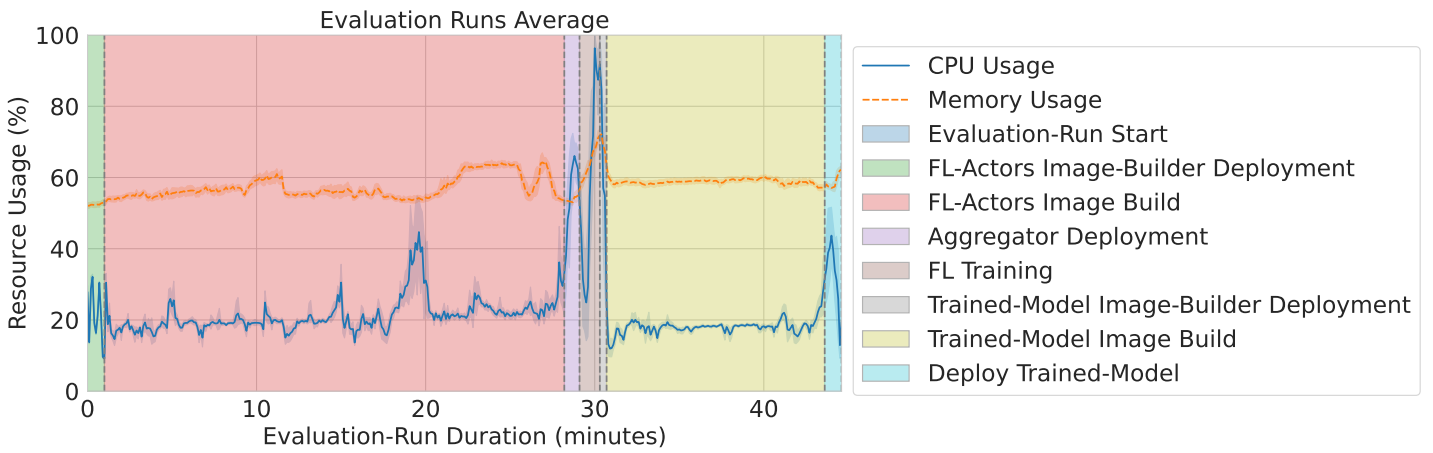
Figure 5.12.: Experiment 4: CPU & Memory Utilization
