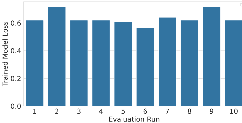
Figure 5.9.: Experiment 1: Trained Model Loss
