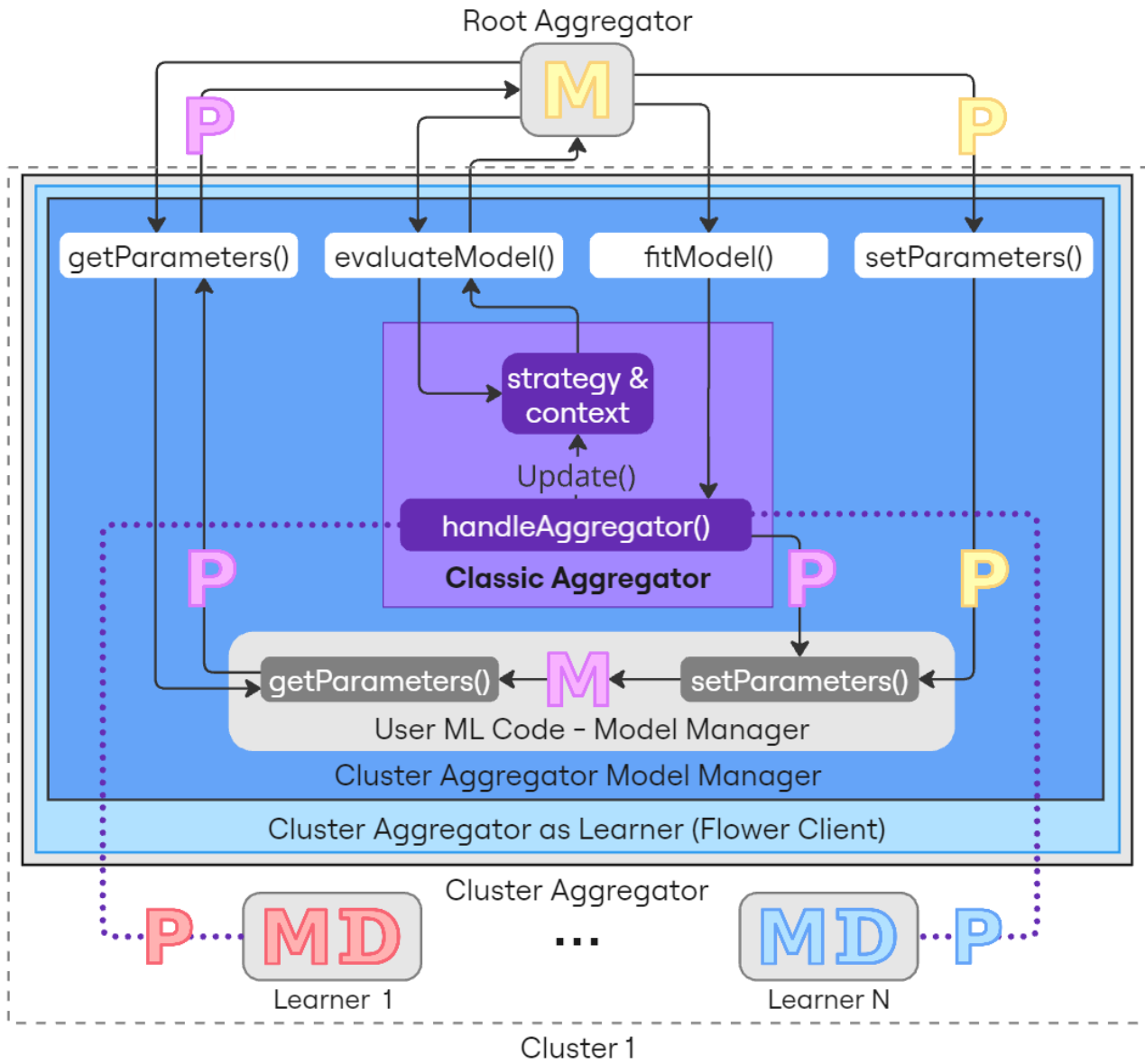
Figure 4.10.: FLOps clustered HFL Architecture
