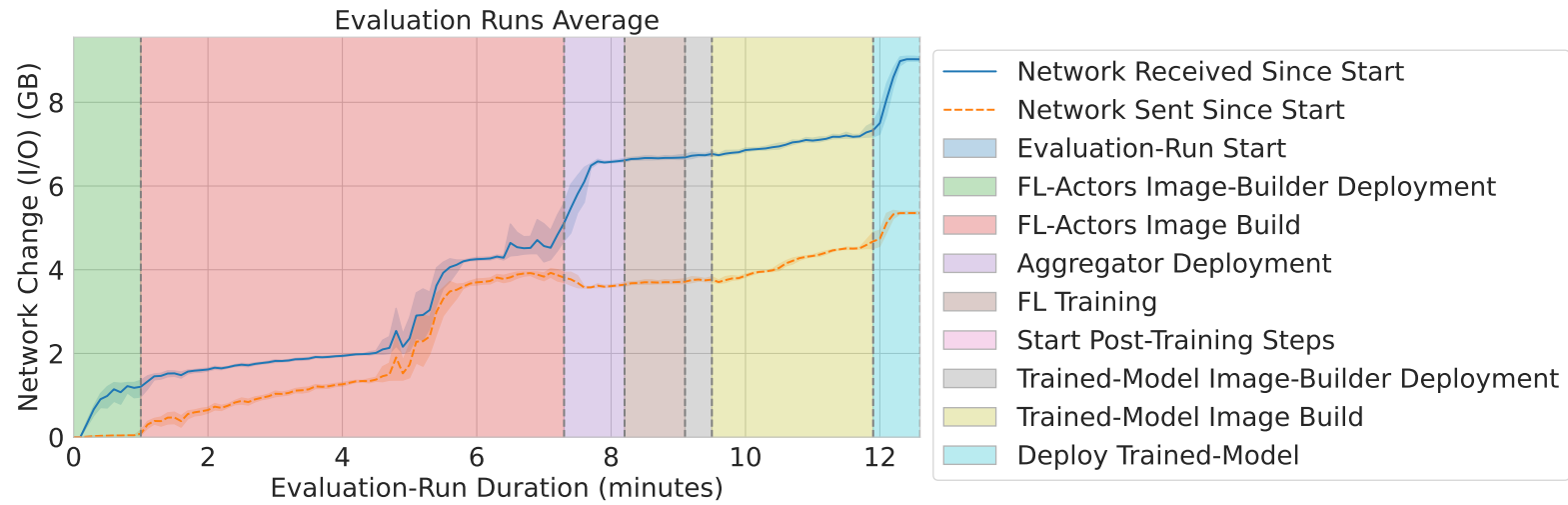
Figure 5.6.: Experiment 1: Net-IO over Time
