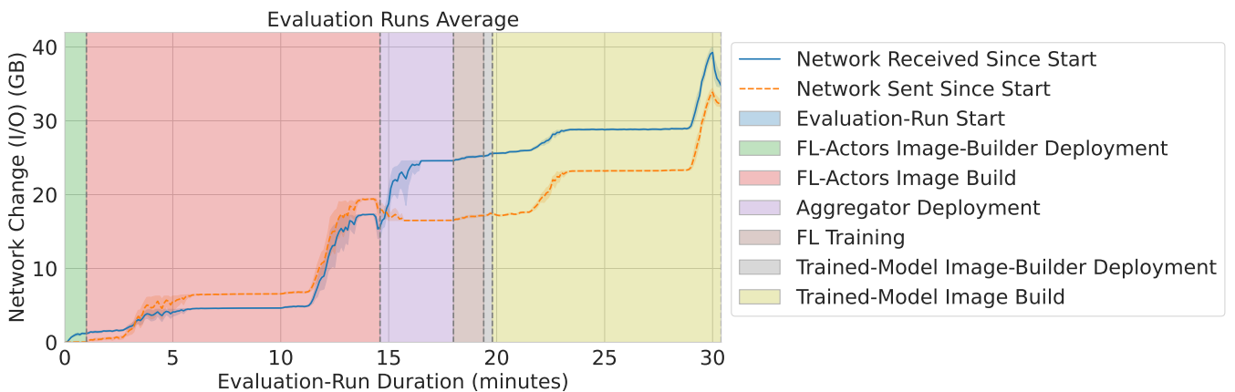
Figure 5.17.: Experiment 5: Network IO
