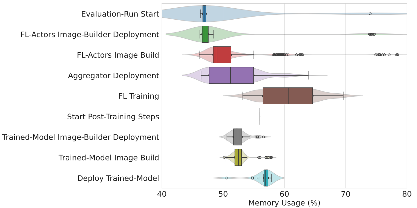
Figure 5.3.: Experiment 1: Memory Utilization by Stage
