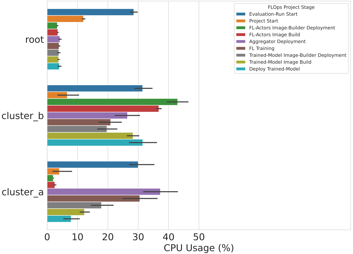
Figure C.10.: Experiment 7: CPU Utilization per Stage
