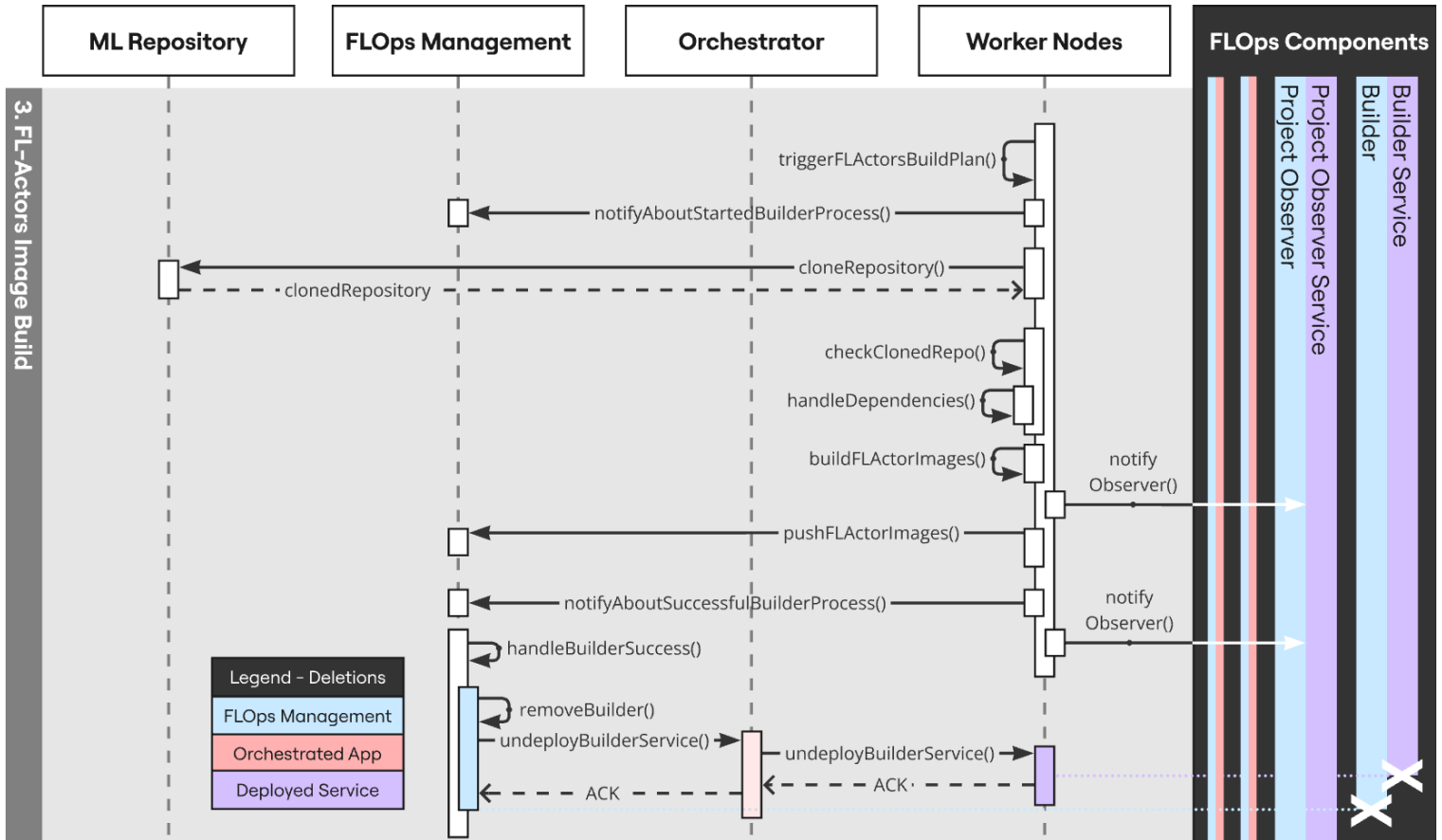
Figure 3.12.: FLOps Image Builder Processes - UML Sequence Diagram
