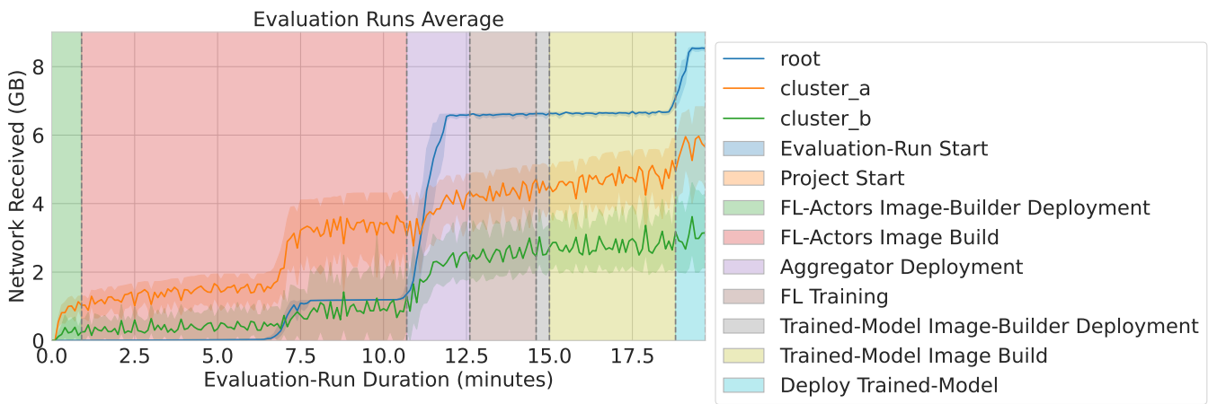
Figure C.14.: Experiment 8: Network Received per Stage
