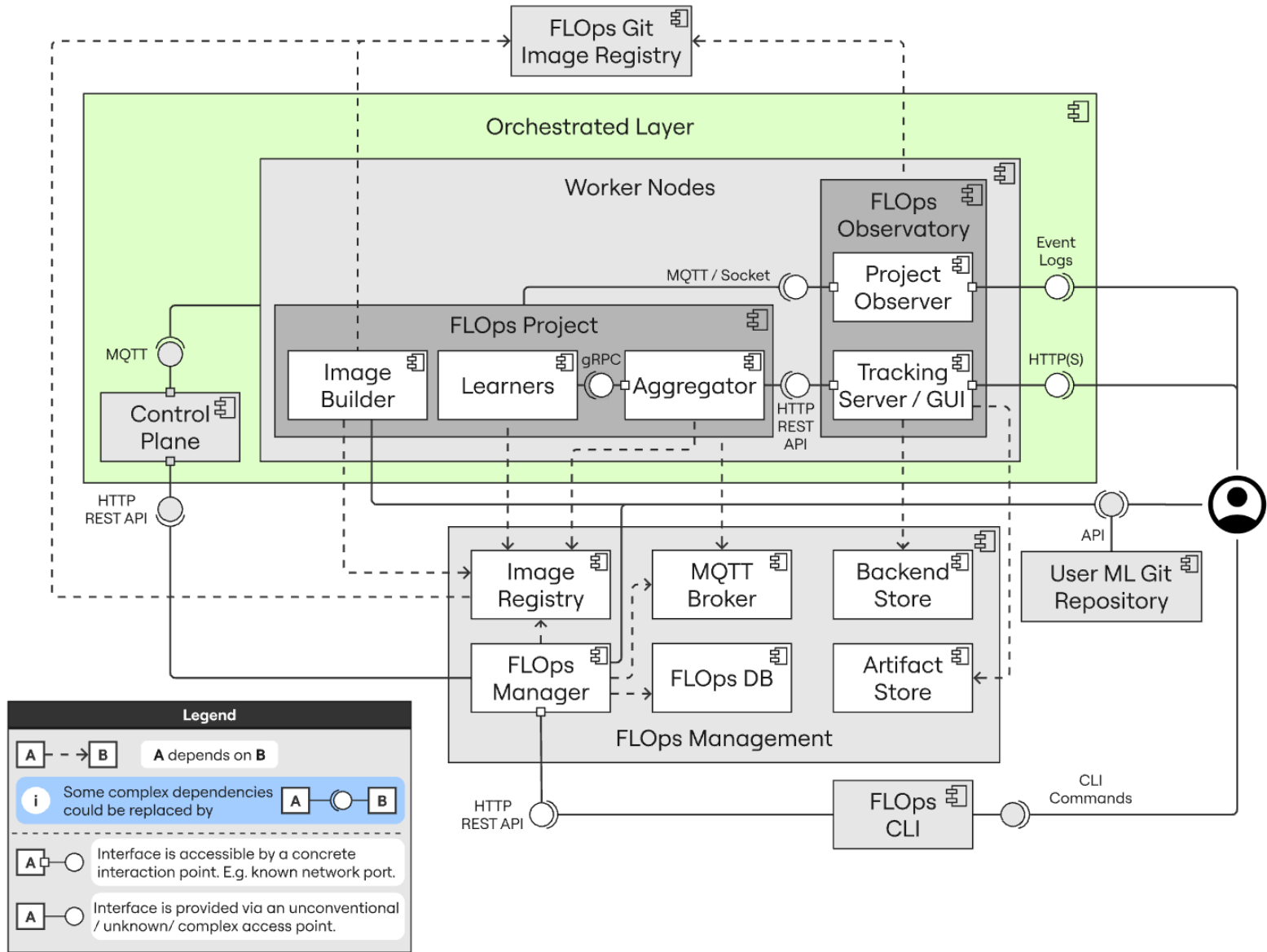
Figure 3.14.: FLOps Subsystem Decomposition
